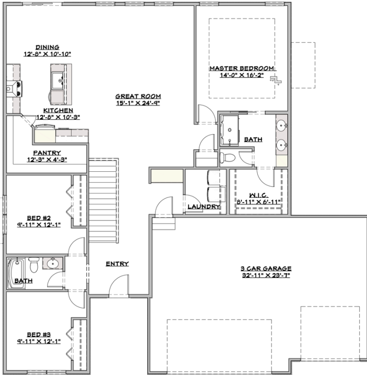
MAIN FLOOR
