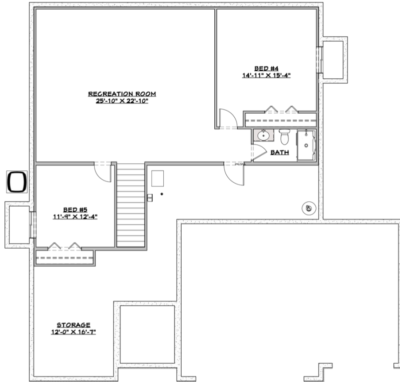
BASEMENT OPTION 4
