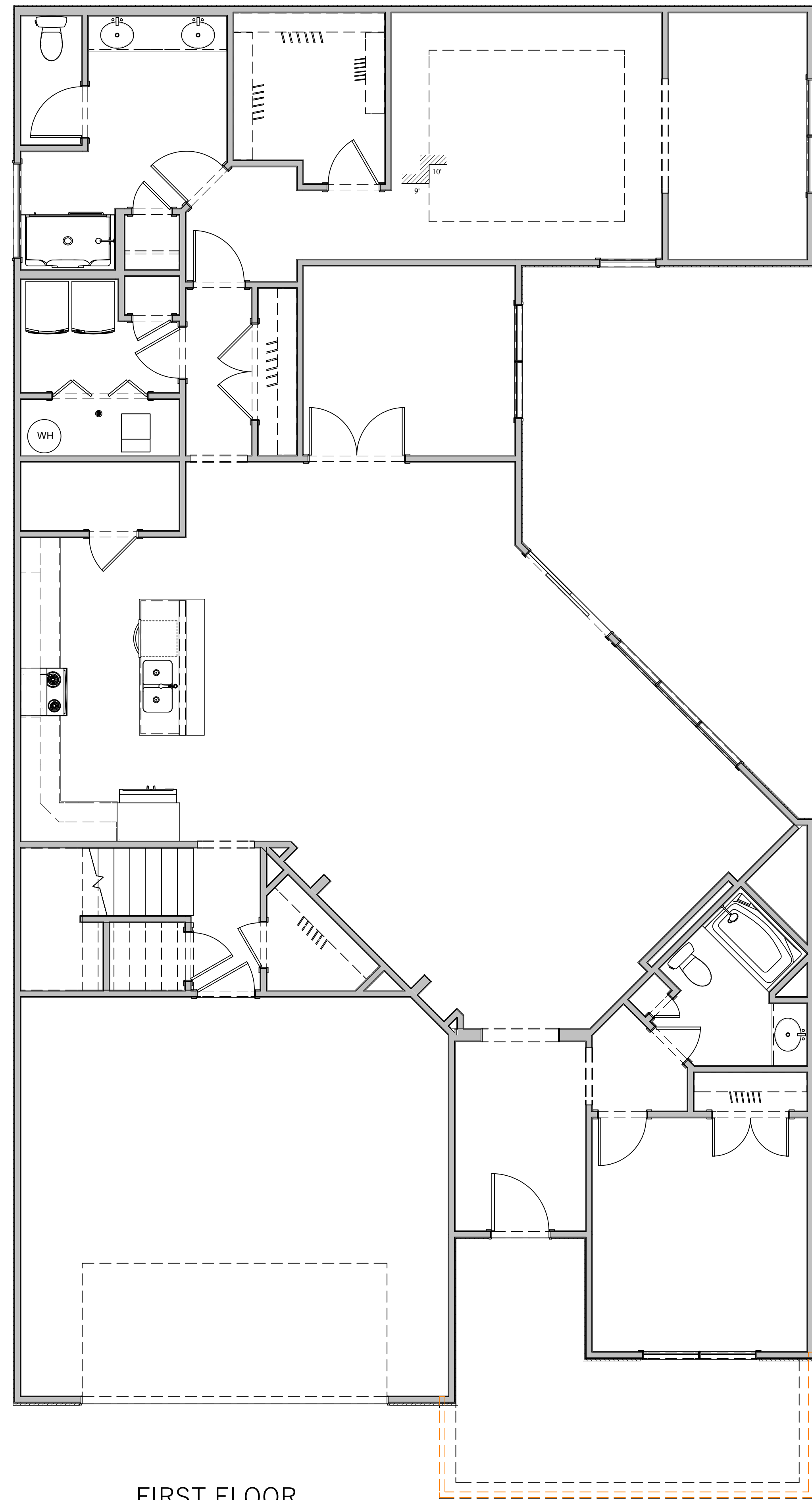
FIRST FLOOR SCALE: 1/4" = 1'-0"
