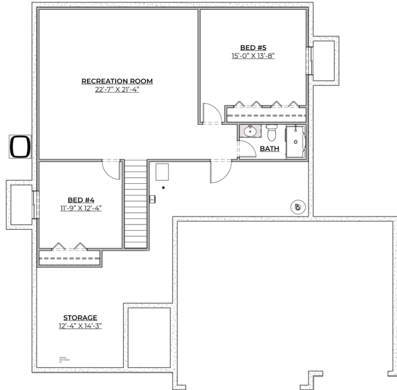
BASEMENT OPTION 4
