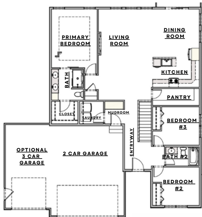
MAIN FLOOR
